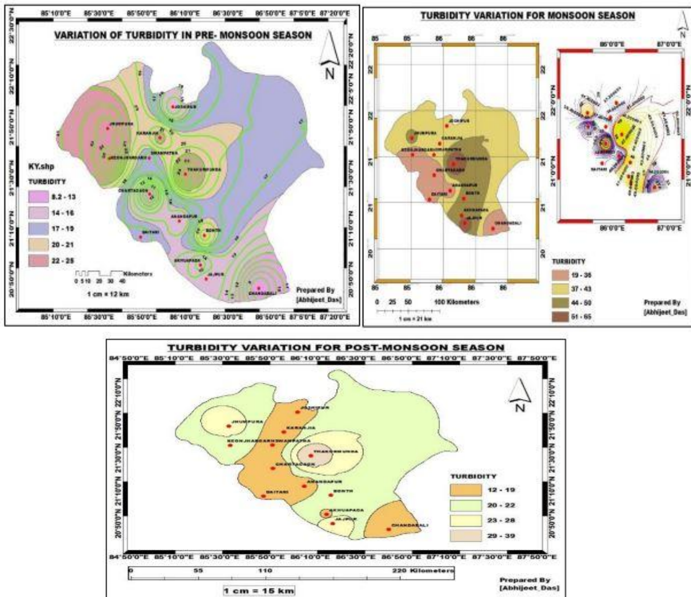
(Figure 6. Spatial variations of turbidity in pre-monsoon, monsoon and post-monsoon season)
