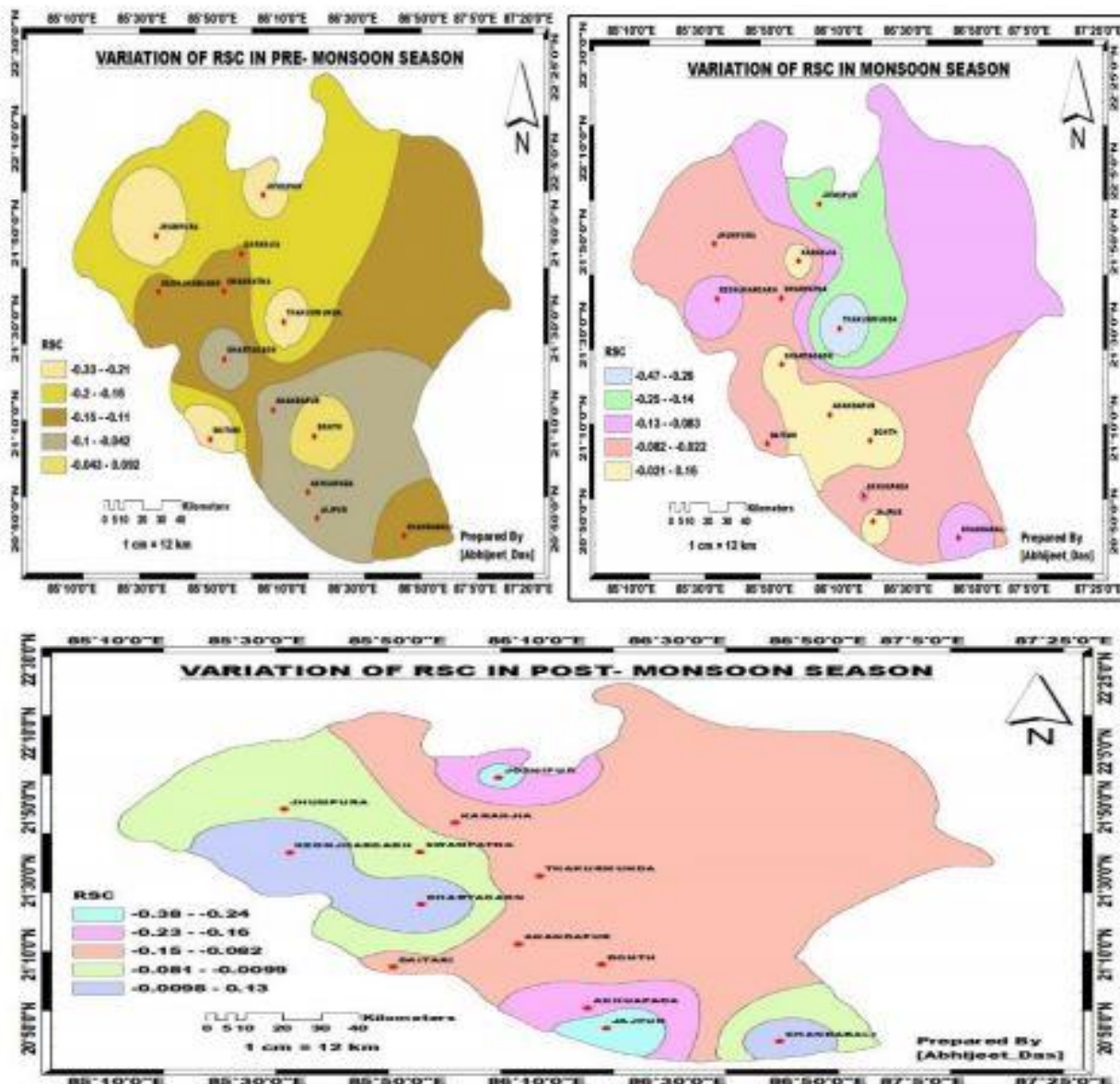
(Figure 32. Spatial variations of RSC in pre-monsoon, monsoon and post-monsoon season)
