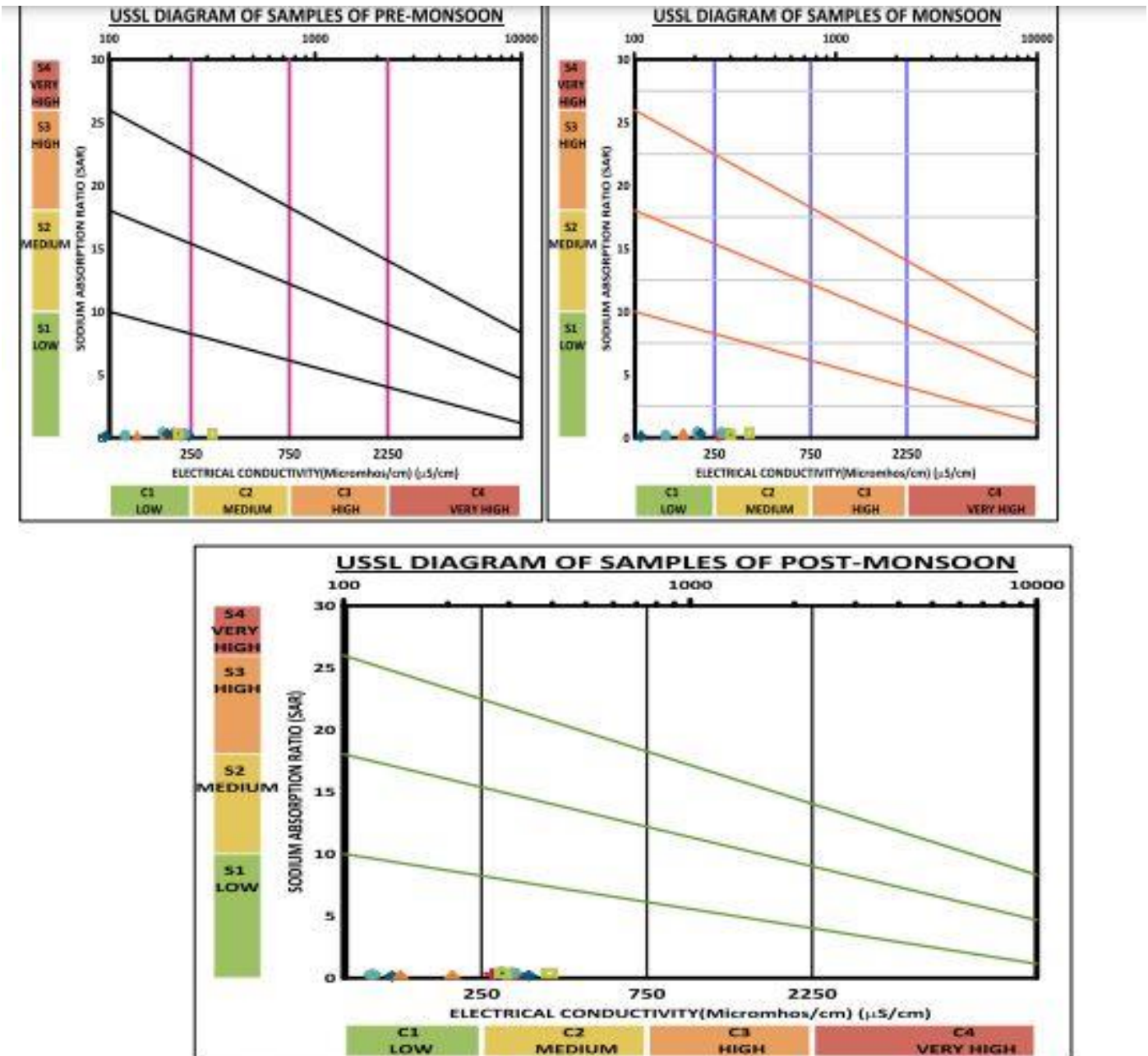
(Figure 29. US Salinity diagrams of pre-monsoon, monsoon and post-monsoon season)
