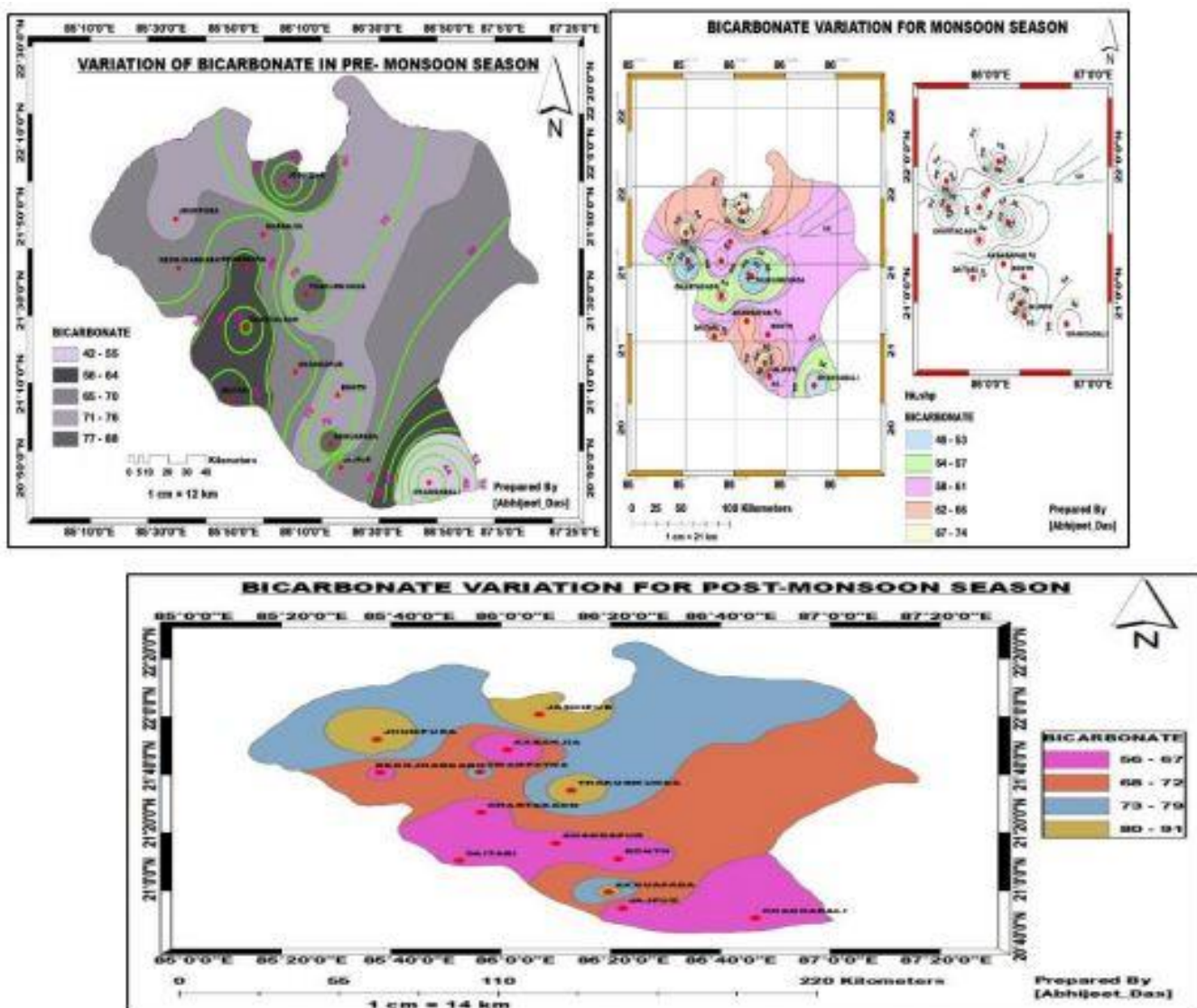
(Figure 19. Spatial variations of bicarbonate in pre-monsoon, monsoon and post-monsoon season)
