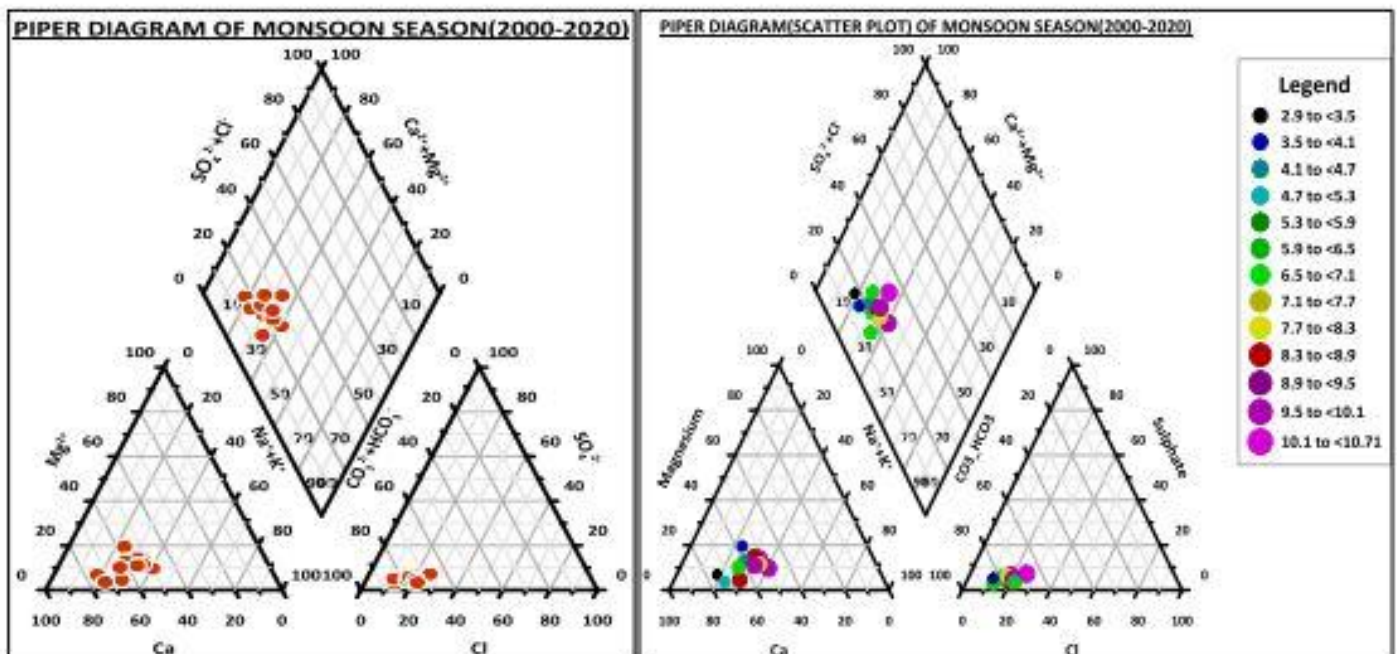
(Figure 37. Piper Diagram for monsoon season)
