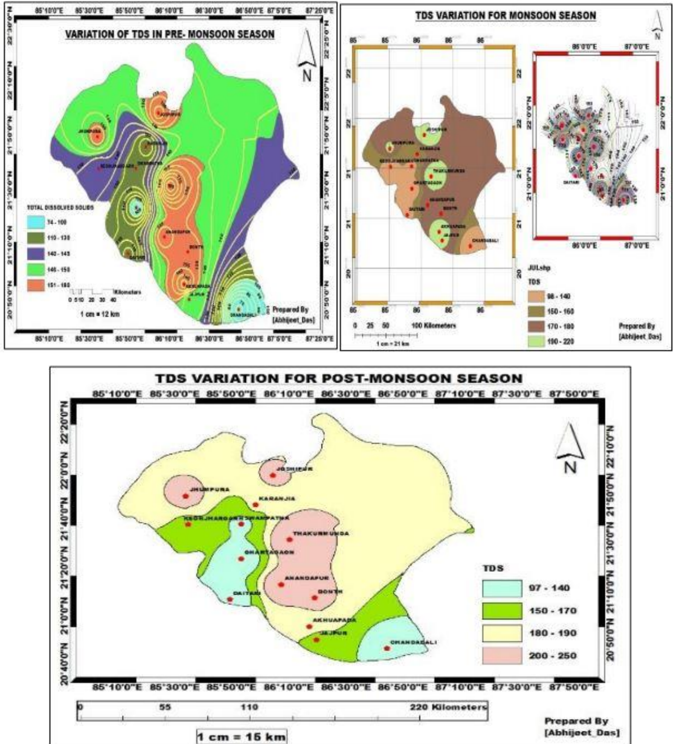
(Figure 7. Spatial variations of TDS in pre-monsoon, monsoon and post-monsoon season)
