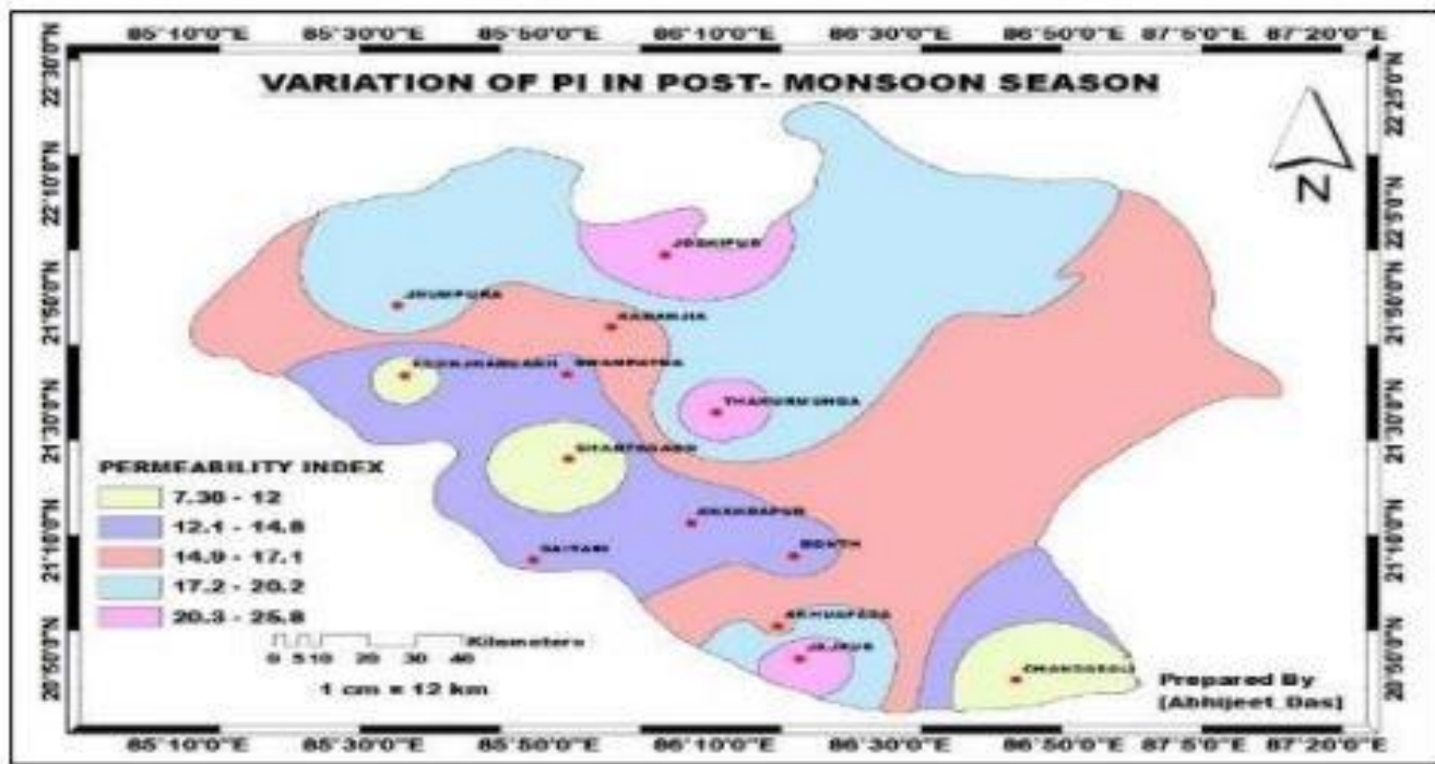
Figure 35. Spatial variations of Permeability Index in pre-monsoon and post-monsoon season)
