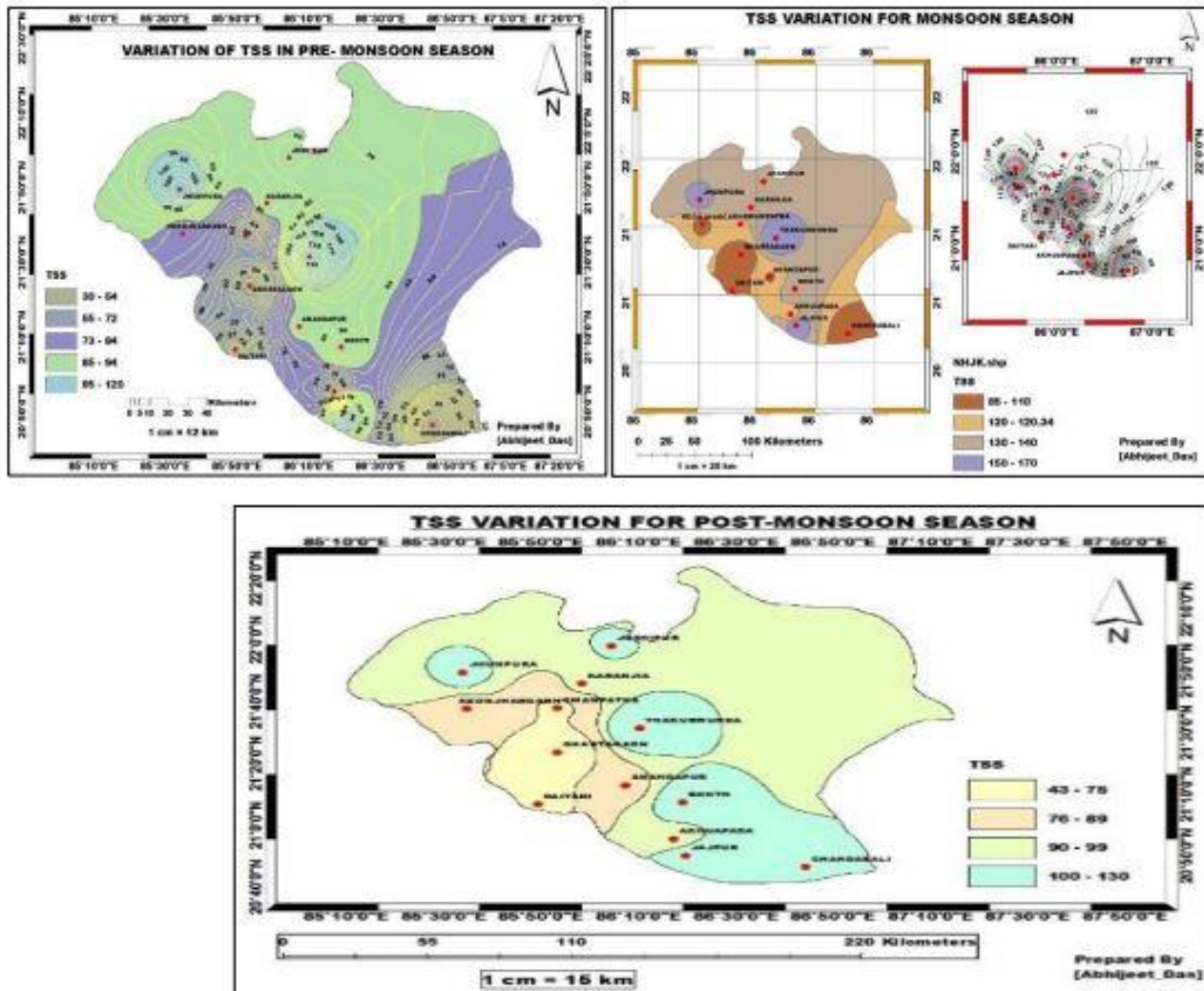
(Figure 8. Spatial variations of TSS in pre-monsoon, monsoon and post-monsoon season)
