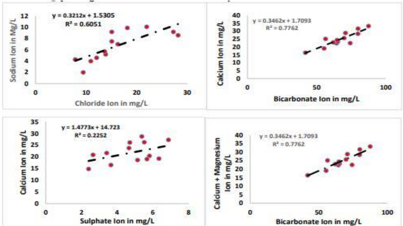
(Figure 26. Relative ionic plots in pre-monsoon season)
