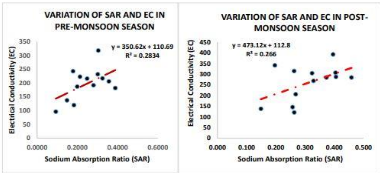
(Figure 31. Correlation between SAR and EC in pre-monsoon and post-monsoon season)
