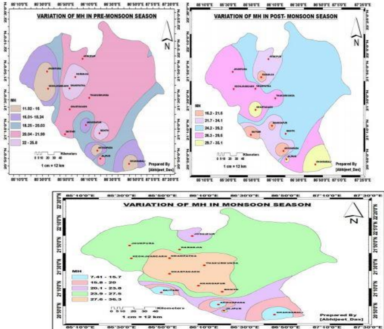
(Figure 33. Spatial variations of MH in pre-monsoon, monsoon and post-monsoon season)
