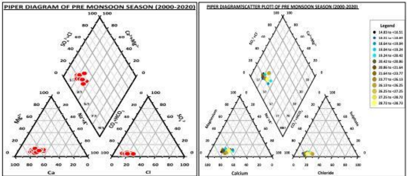
(Figure 36. Piper Diagram for Pre-monsoon season)
