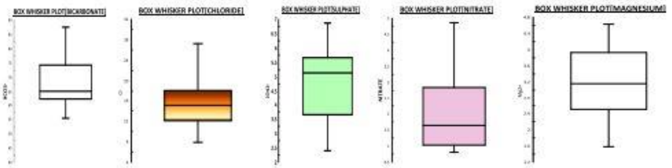
(Figure 24.Box plot of pre-monsoon analysis)
