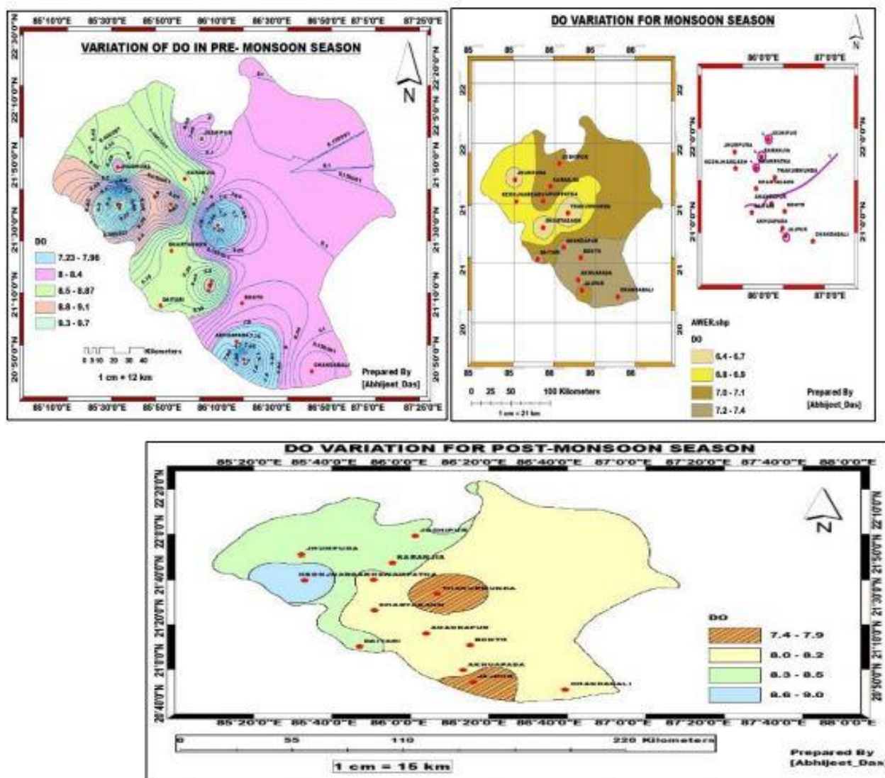
(Figure 10. Spatial variations of DO in pre-monsoon, monsoon and post-monsoon season)
