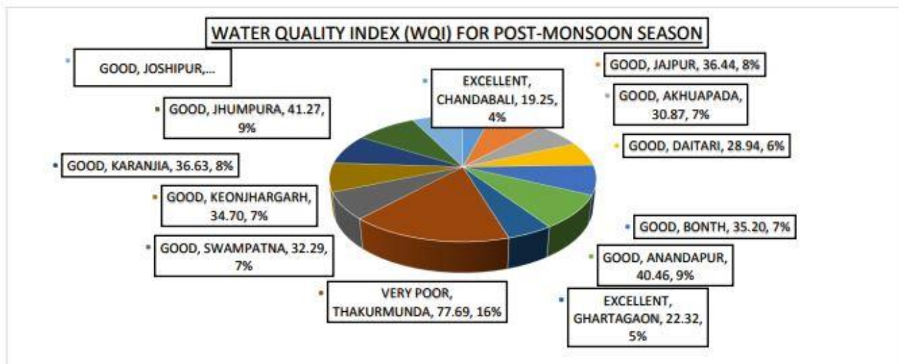
(Figure 43. Water Quality Index (WQI) variation as shown in pie charts for pre-monsoon, monsoon and post-monsoon season)
