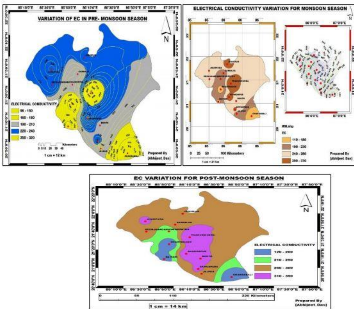
(Figure 9. Spatial variations of EC in pre-monsoon, monsoon and post-monsoon season)
