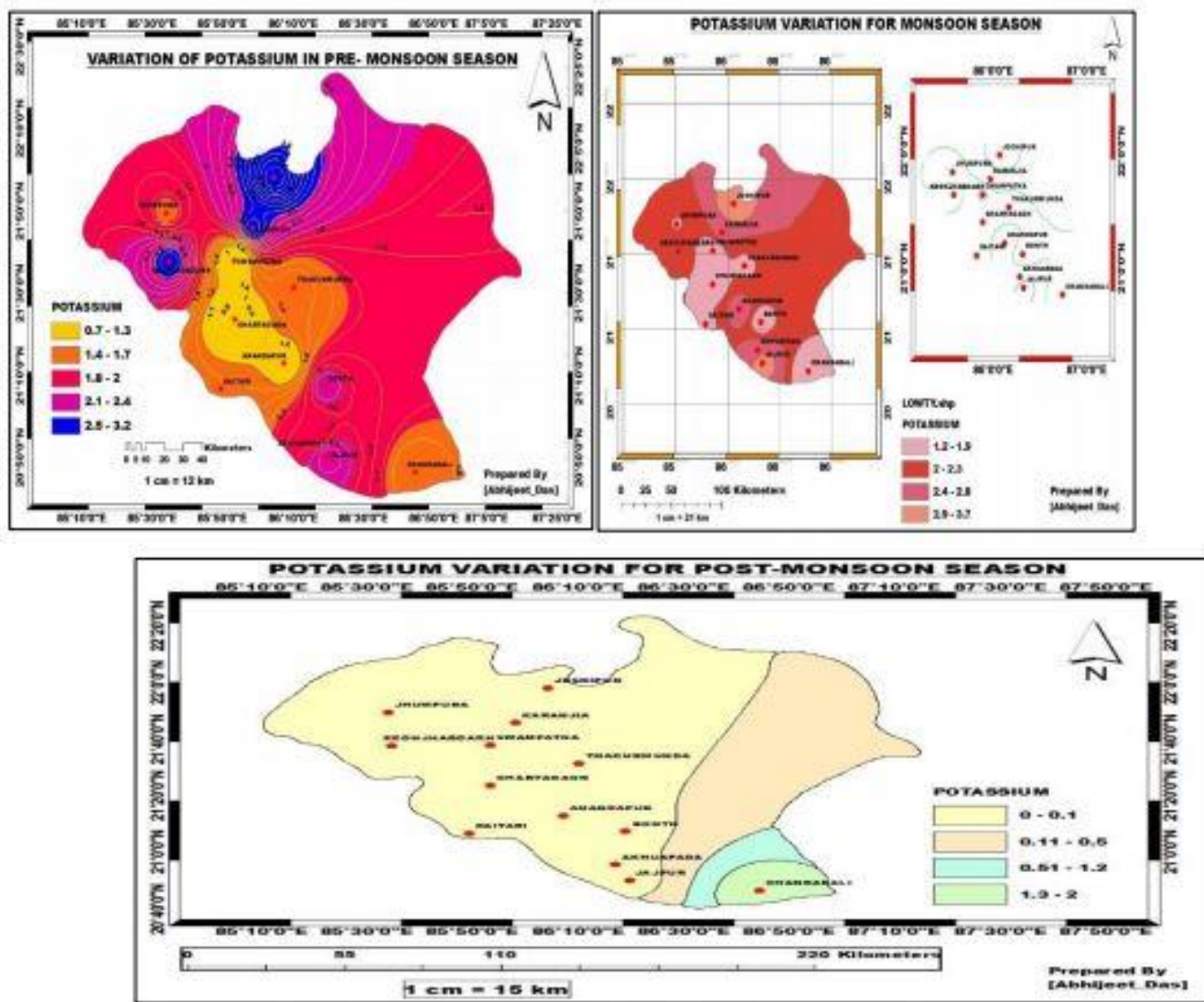
(Figure 18. Spatial variations of potassium in pre-monsoon, monsoon and post-monsoon season)
