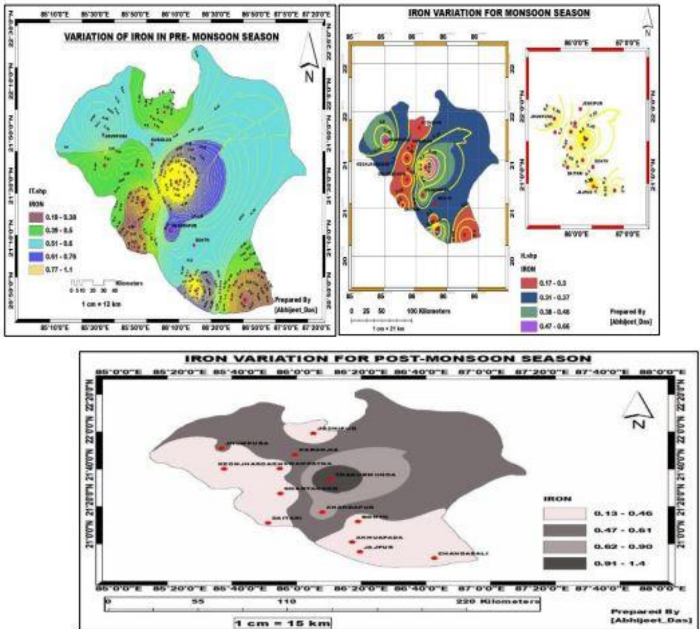
(Figure 16. Spatial variations of iron in pre-monsoon, monsoon and post-monsoon season)
