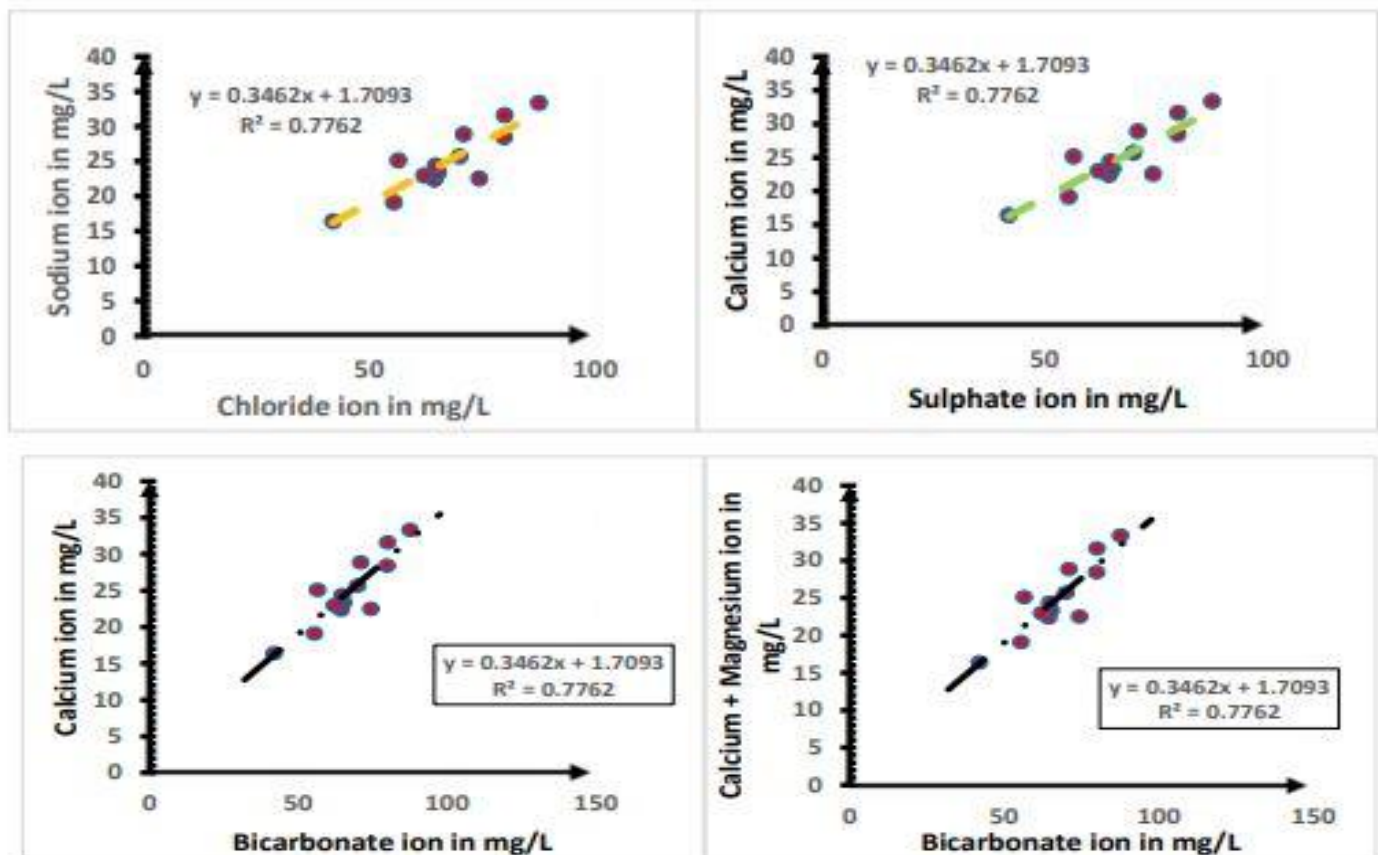
(Figure 27. Relative ionic plots in post-monsoon season)
