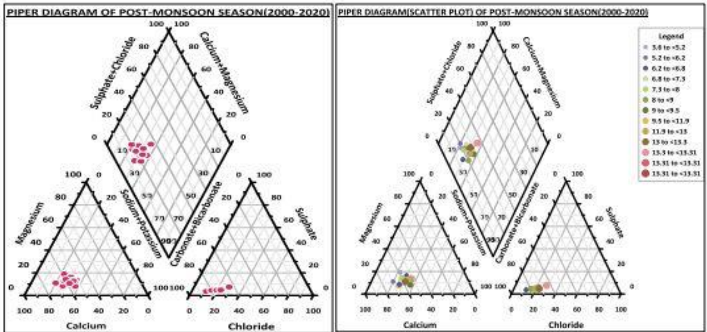
(Figure 38. Piper Diagram for Post-monsoon season)
