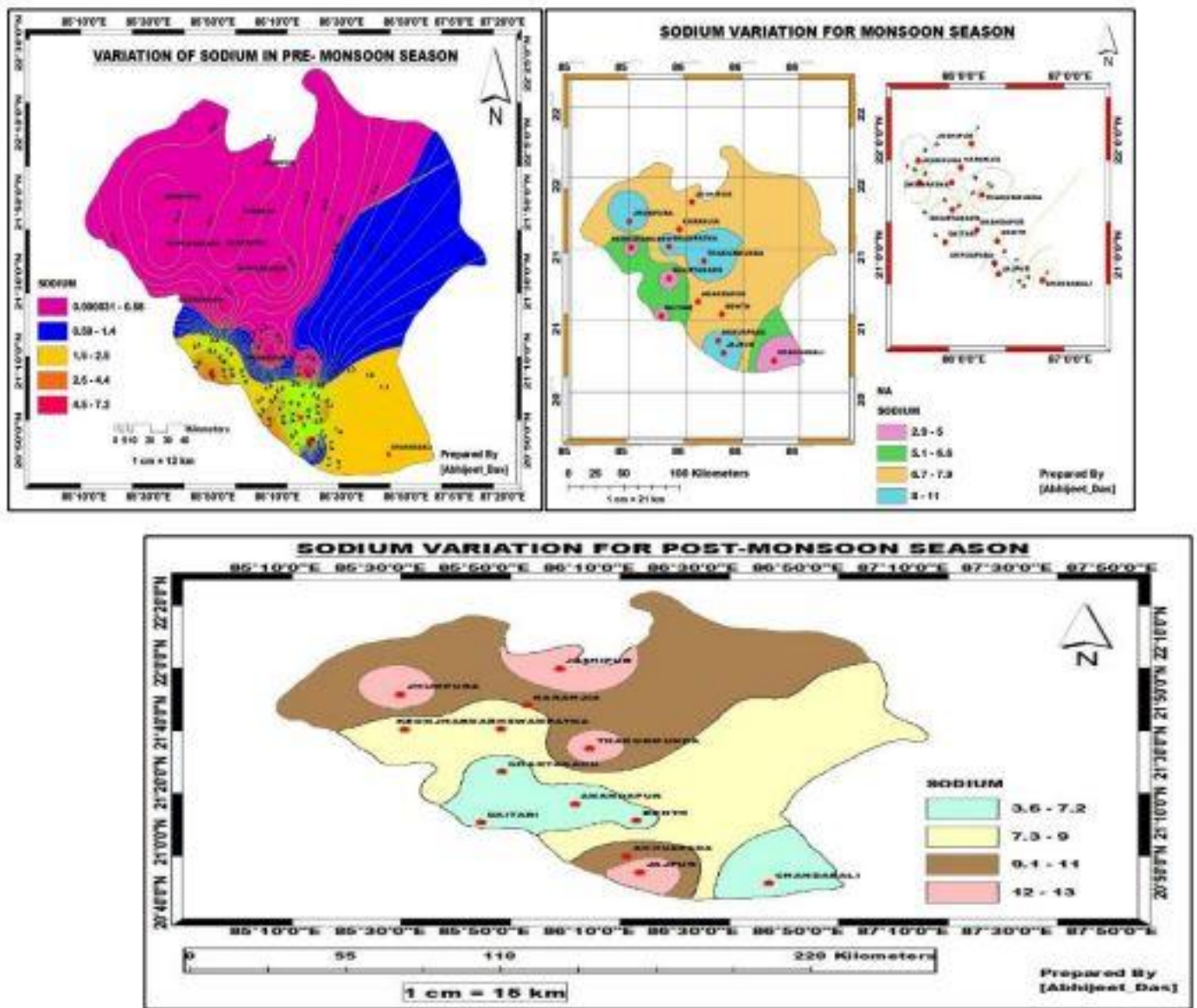
(Figure 17. Spatial variations of sodium in pre-monsoon, monsoon and post-monsoon season)
