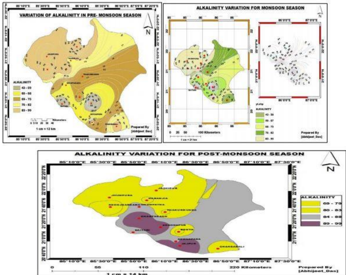
(Figure 11. Spatial variations of alkalinity in pre-monsoon, monsoon and post-monsoon season)
