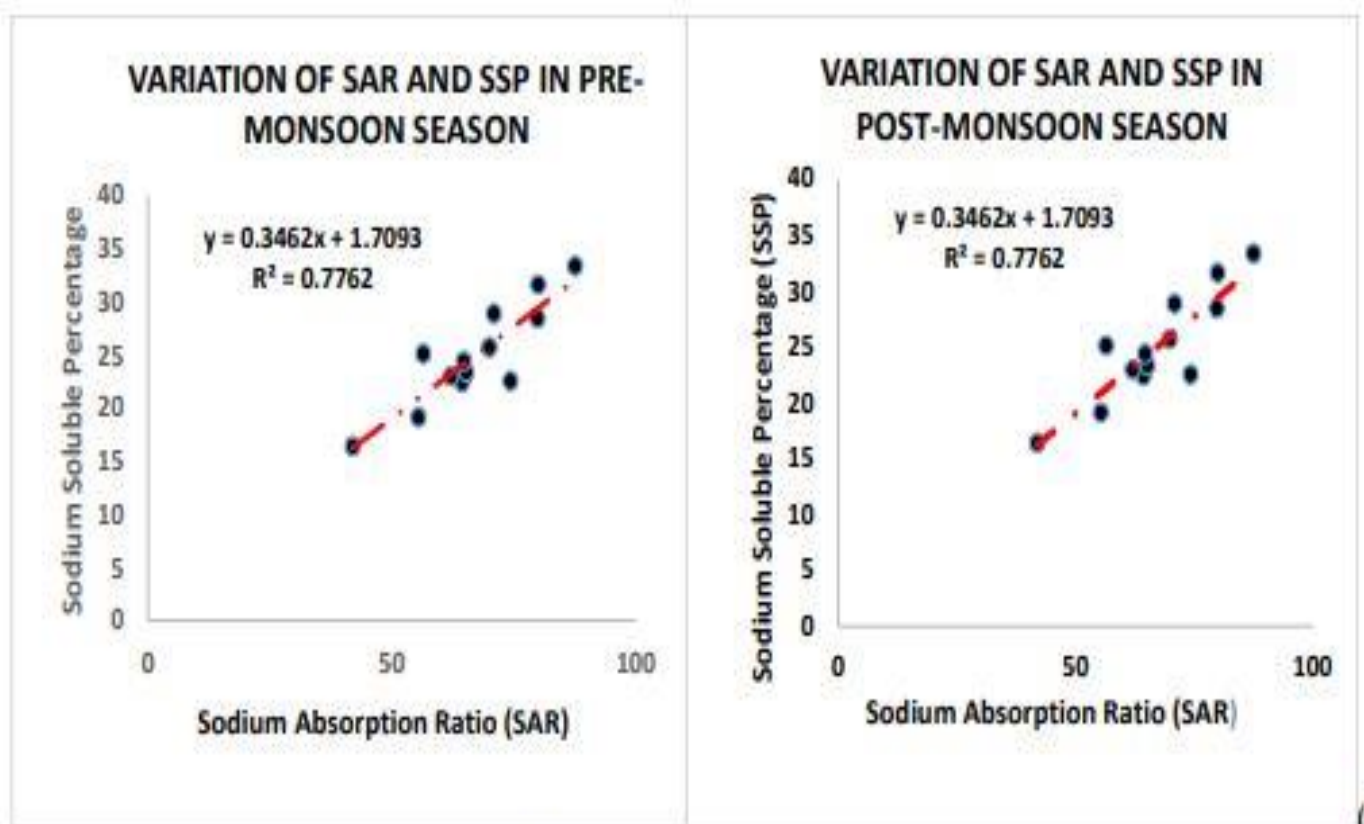
Correlation between SAR and SSP in pre-monsoon and post-monsoon season)
