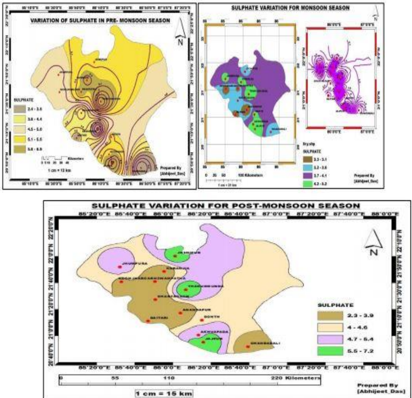
(Figure 21. Spatial variations of sulphate in pre-monsoon, monsoon and post-monsoon season)
