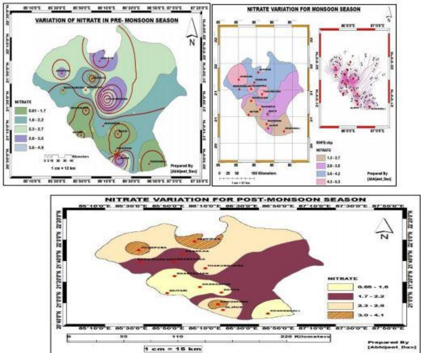
(Figure 23. Spatial variations of nitrate in pre-monsoon, monsoon and post-monsoon season)
